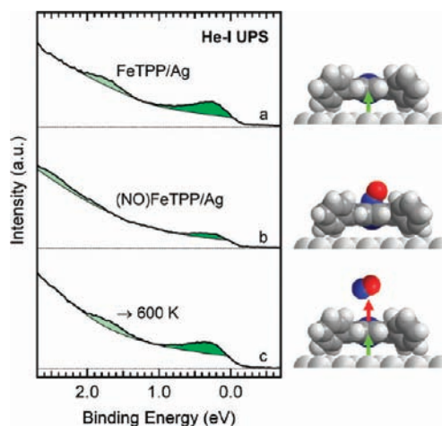
Figure 6. Valence electronic structure of FeTPP and (NO)FeTPP on Ag(111): He–I UP spectra of (a) FeTPP monolayer, (b) (NO)FeTPP monolayer, and (c) after heating the (NO)FeTPP monolayer to 600 K for removal of the NO ligand.
