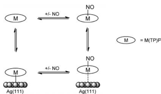
Figure 9. Transformations considered in the theoretical analysis, M = Fe, Co, Zn. In the periodic slab calculations, the MTPP molecules are modeled as metalloporphyrins MP (i.e., by omitting the peripheral phenyl rings) adsorbed to a five-layer Ag slab (see Section 2 for details). In the molecular model systems, calculations with the full MTPPs have been performed, but the Ag(111) surface has been replaced by a single Ag atom. See Tables 1 and 3 for structural data and Tables 2 and 4 for associated binding energies.
