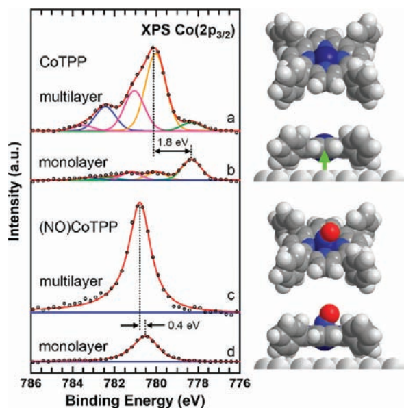
Figure 1. Co(2p 3/2 ) XP spectra of CoTPP and (NO)CoTPP on Ag(111): (a) CoTPP multilayers (~4 layers), (b) CoTPP monolayer, (c) (NO)CoTPP multilayers (~4 layers), and (d) (NO)CoTPP monolayer. The small shoulder around 778 eV in (a) stems from the CoTPP monolayer. The other curves in the signal deconvolution of (a) and (c) are displayed for illustrative purposes and do not necessarily represent the full complexity of the spectra.
