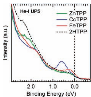
Figure 7. Comparison of the He-I UPS spectra of CoTPP (blue), FeTPP (red), ZnTPP (green), and 2HTPP (black, dashed).
