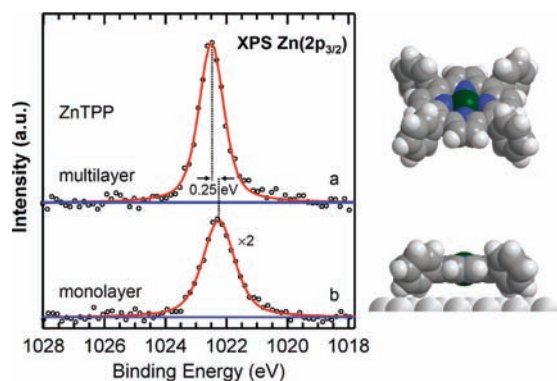
Figure 4. Zn( 2p_{3/2} ) XP spectra of (a) multilayers and (b) monolayer of ZnTPP on Ag(111).
