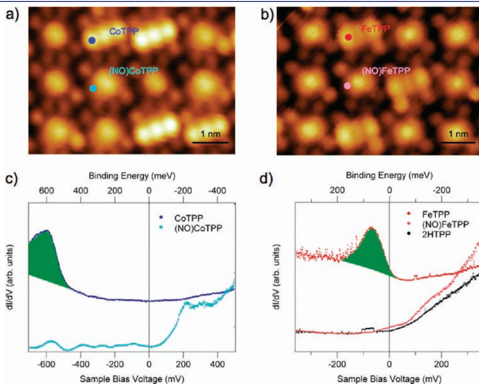
Figure 8. Scanning tunneling microscopy (STM) images and ST spectra of MTPP and (NO)MTPP on Ag(111) showing the quenching of the interaction-induced peak (marked in green) upon NO coordination. (a) STM image of a mixed CoTPP and (NO)CoTPP array ( I = 55 \text{ pA} , V = -0.7 \text{ V} ). The NO related species are characterized by a round central protrusion. The colored dots represent the off-center position above the porphyrin macrocycle where ST spectra were recorded (compare c and d), see text for discussion). (b) Mixed FeTPP and (NO)FeTPP array ( I = 0.1 \text{ nA} , V = -0.7 \text{ V} ). (c) ST spectra of CoTPP (blue) and (NO)CoTPP (light blue), compare to the UP spectra in Figure 5. (Stabilizing parameters for the STM tip before opening the feedback loop: I = 55 \text{ pA} , V = -0.6 \text{ V} , modulation amplitude 25 mV, modulation frequency 967 Hz.) (d) ST spectra of FeTPP (red), (NO)FeTPP (light red) and 2HTPP (black) on Ag(111), compare to Figure 6 ( I = 0.2 \text{ nA} , V = -0.28 \text{ V} , modulation amplitude 25 mV, modulation frequency 398 Hz).
