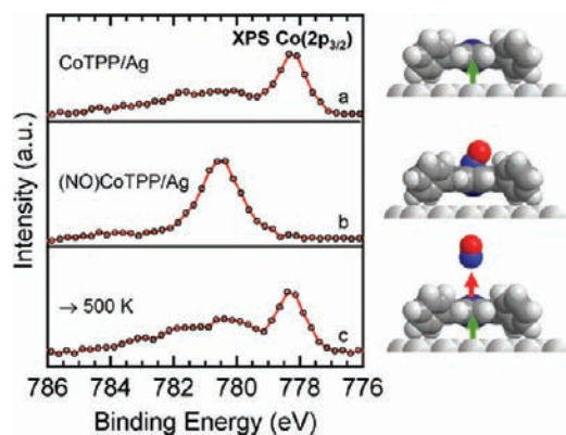
Figure 2. Reversibility of the changes in the electronic structure induced by NO coordination: Co(2p 3/2 ) XP spectra of CoTPP and (NO)CoTPP on Ag(111). (a) CoTPP monolayer, (b) (NO)CoTPP monolayer, (c) after heating the (NO)CoTPP monolayer to 500 K for thermal desorption of the NO ligand.
